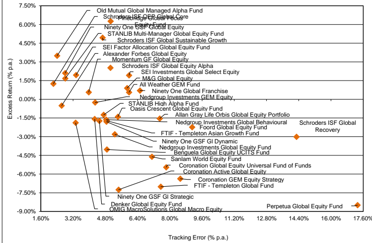
Excess Return vs Tracking Error Scatterplot - Global Equity 3 Years ended 30 November 2022
