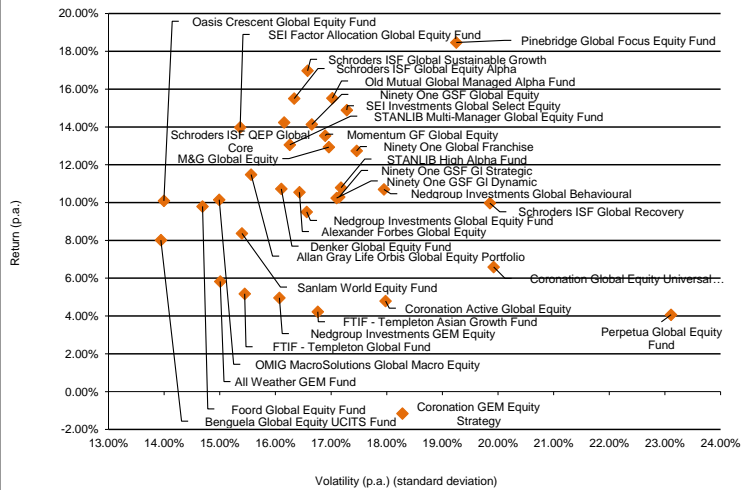
Volatility vs Return Scatterplot - Global Equity 3 Years ended 30 November 2022
