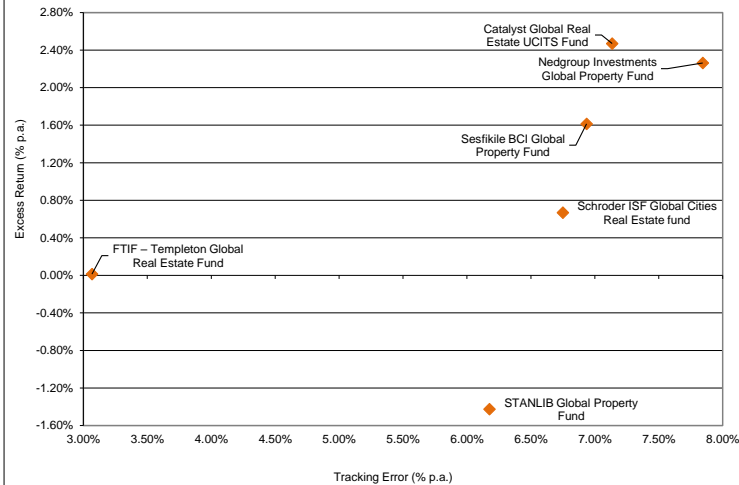
Excess Return vs Tracking Error Scatterplot - Global Property 3 Years ended 30 November 2022
