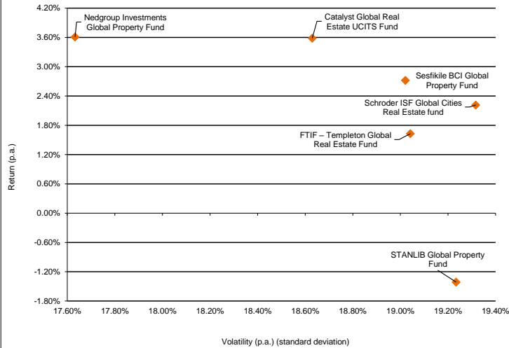
Volatility vs Return Scatterplot - Global Property 3 Years ended 30 November 2022
