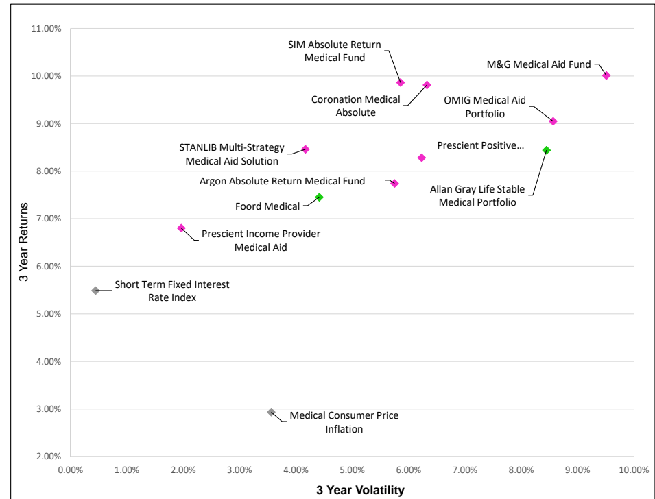
Volatility-Return Scatterplot of Medical Aid Managers - Absolute Return and Balanced for 3 Years ended 31 December 2021
