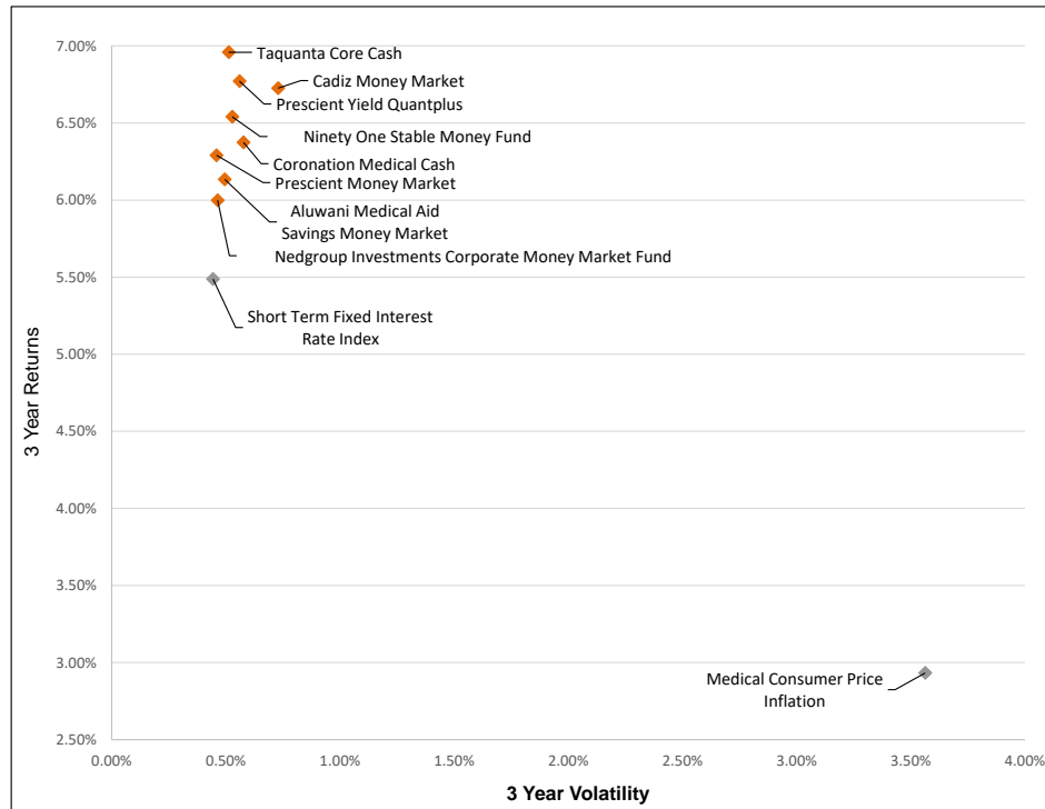
Volatility-Return Scatterplot of Medical Aid Managers - Money Market for 3 Years ended 31 December 2021
