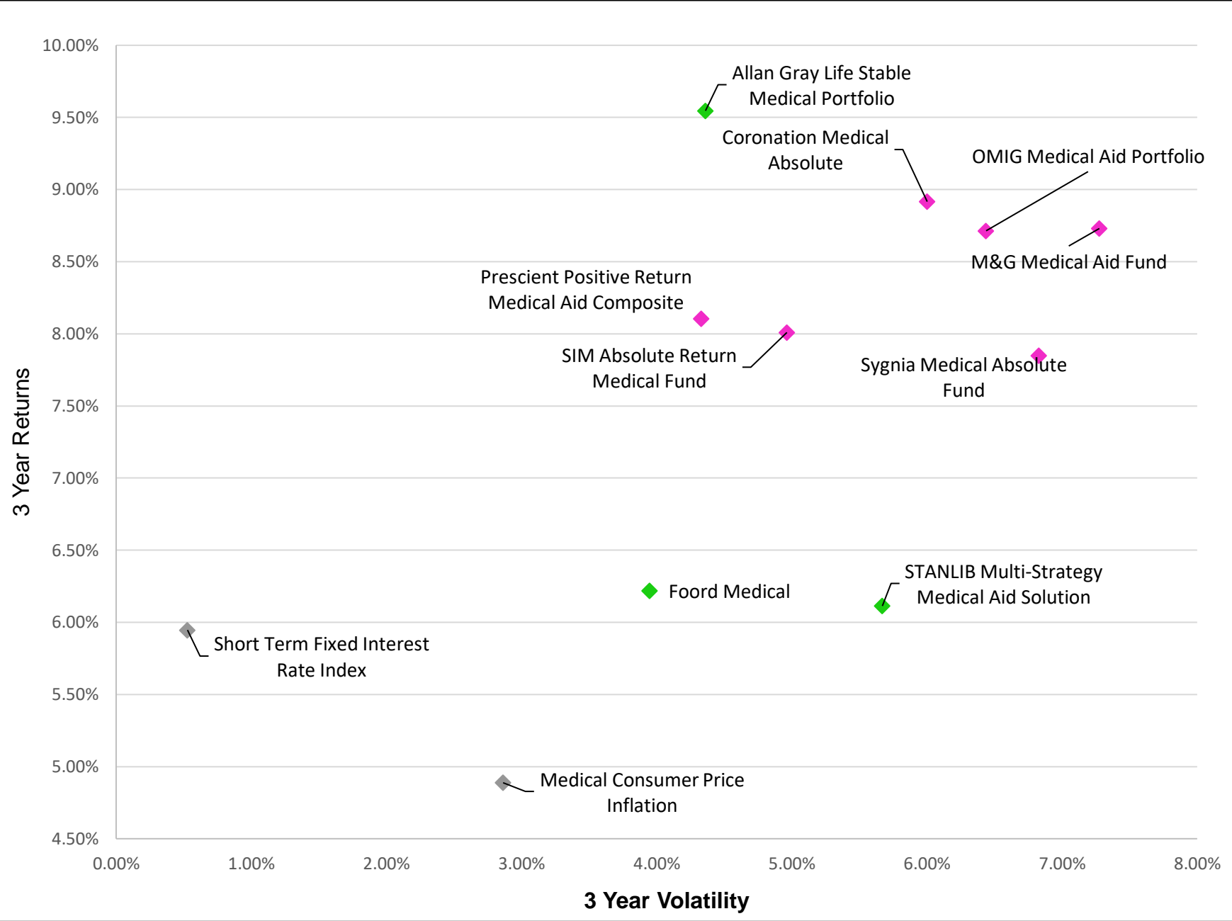
Volatility-Return Scatterplot of Medical Aid Managers - Absolute Return and Balanced for 3 Years ended 29 February 2024
