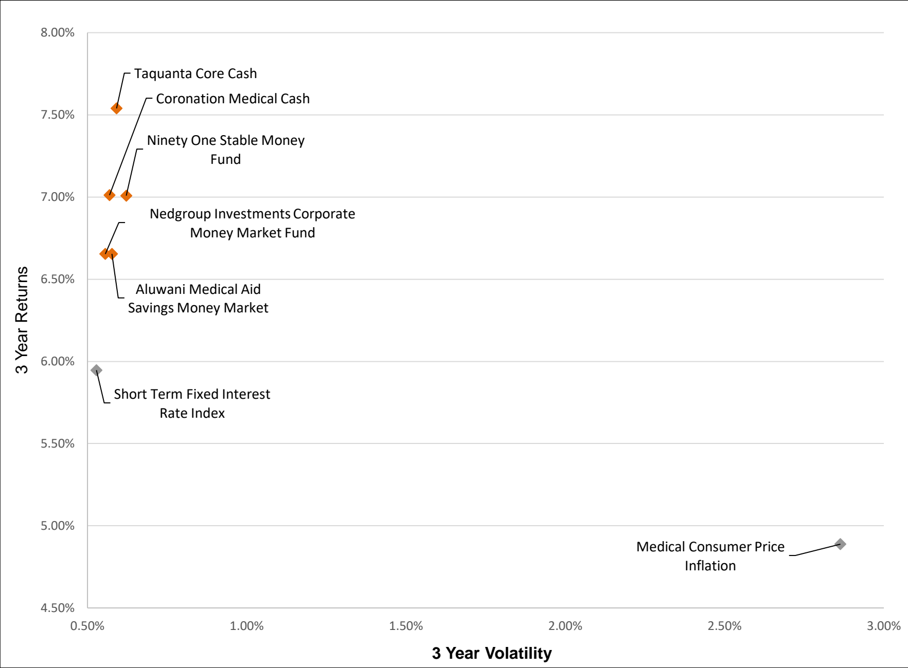
Volatility-Return Scatterplot of Medical Aid Managers - Money Market for 3 Years ended 29 February 2024
