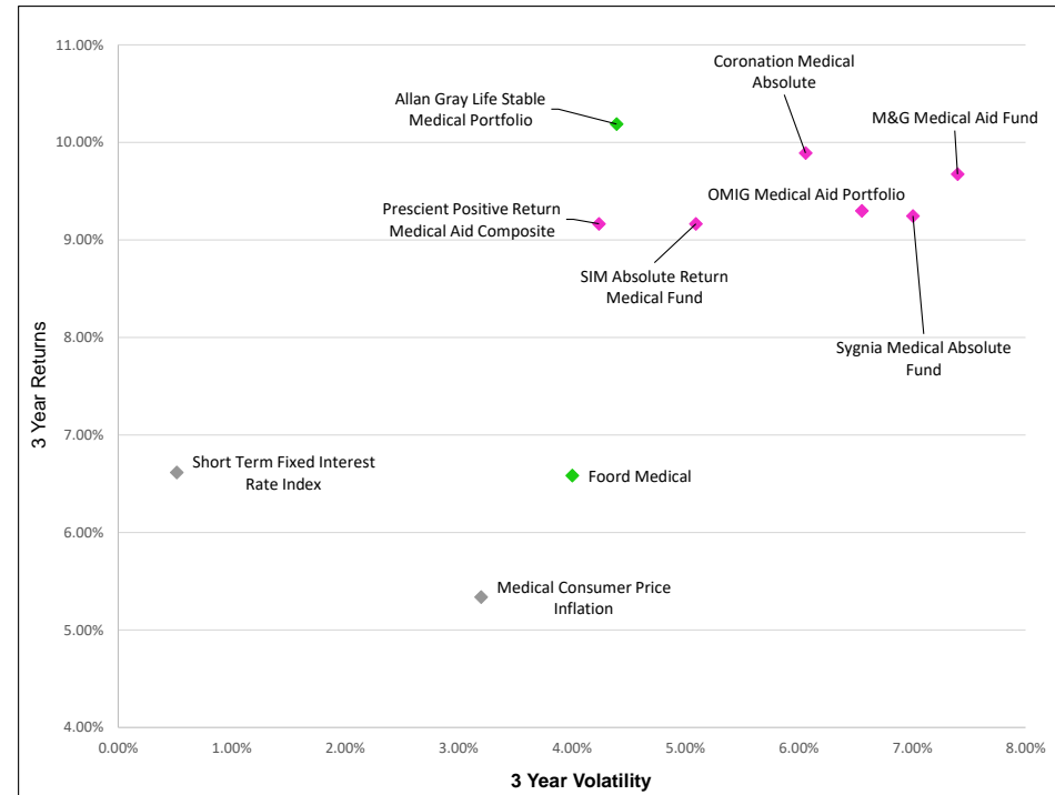
Volatility-Return Scatterplot of Medical Aid Managers - Absolute Return and Balanced for 3 Years ended 31 July 2024
