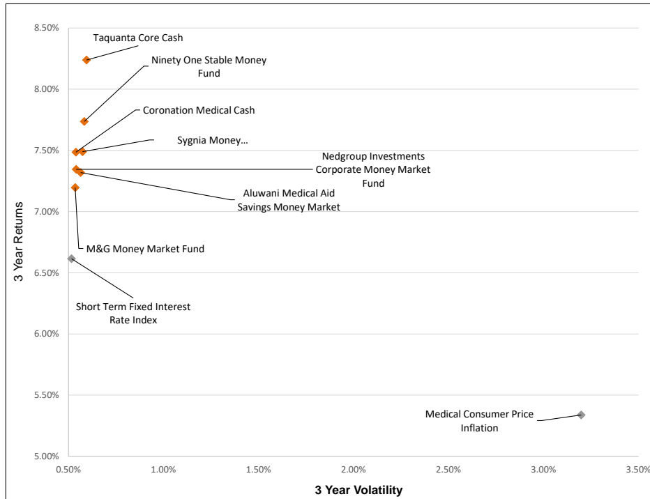
Volatility-Return Scatterplot of Medical Aid Managers - Money Market for 3 Years ended 31 July 2024
