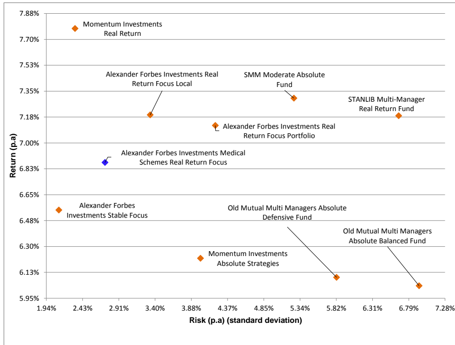
Volatility vs Return Scatterplot - Multi Managers Absolute Return and Medical Aid funds 3 Years ended 30 April 2019
