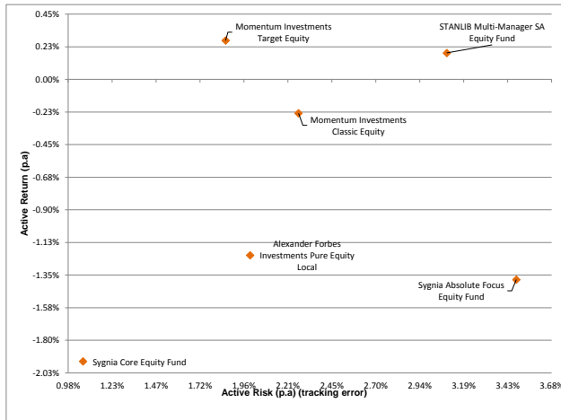
Excess Return vs Tracking Error Scatterplot - Multi Managers Equity 3 Years ended 30 April 2019
