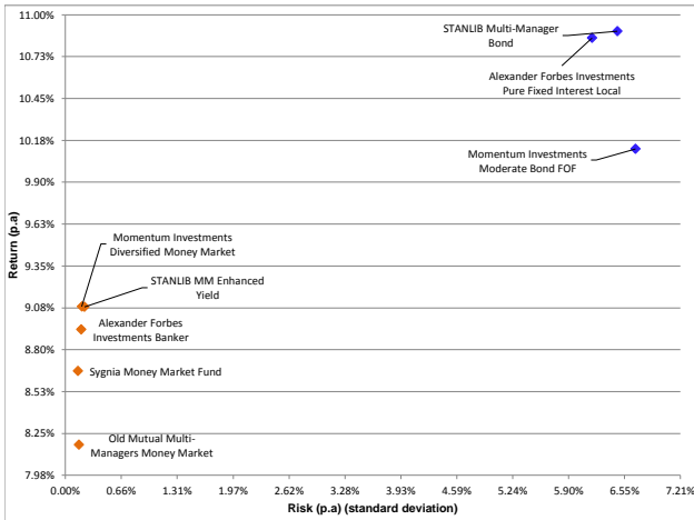
Volatility vs Return Scatterplot - Multi Managers Bonds and Money Market - 3 Years ended 30 April 2019
