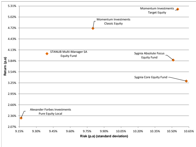
Volatility vs Return Scatterplot - Multi Managers Equity 3 Years ended 30 April 2019
