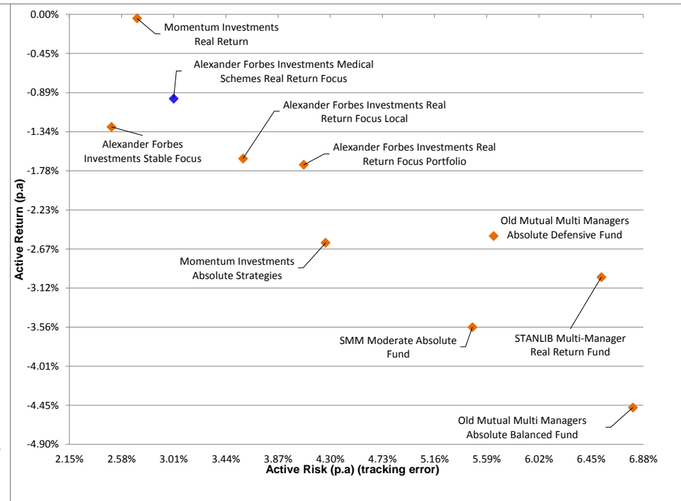
Excess Return vs Tracking Error Scatterplot - Multi Managers Absolute Return and Medical Aid funds 3 Years ended 30 April 2019
