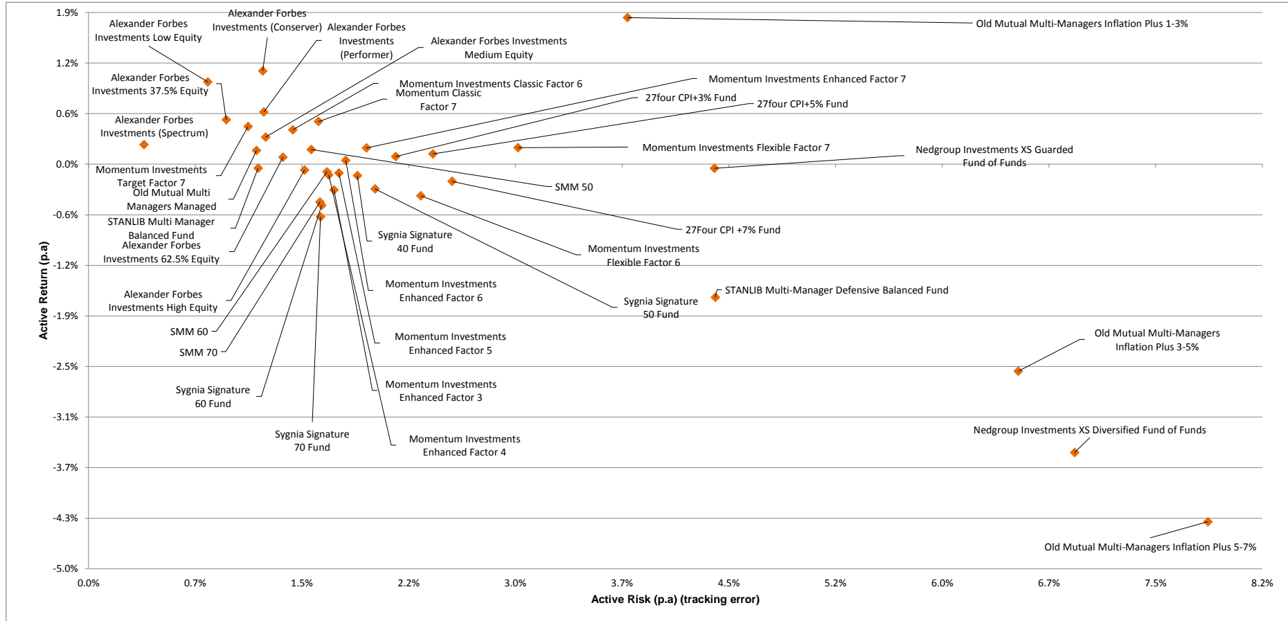
Excess Return vs Tracking Error Scatterplot - Multi Managers Fixed & Strategic Asset Allocation 3 Years ended 30 April 2019
