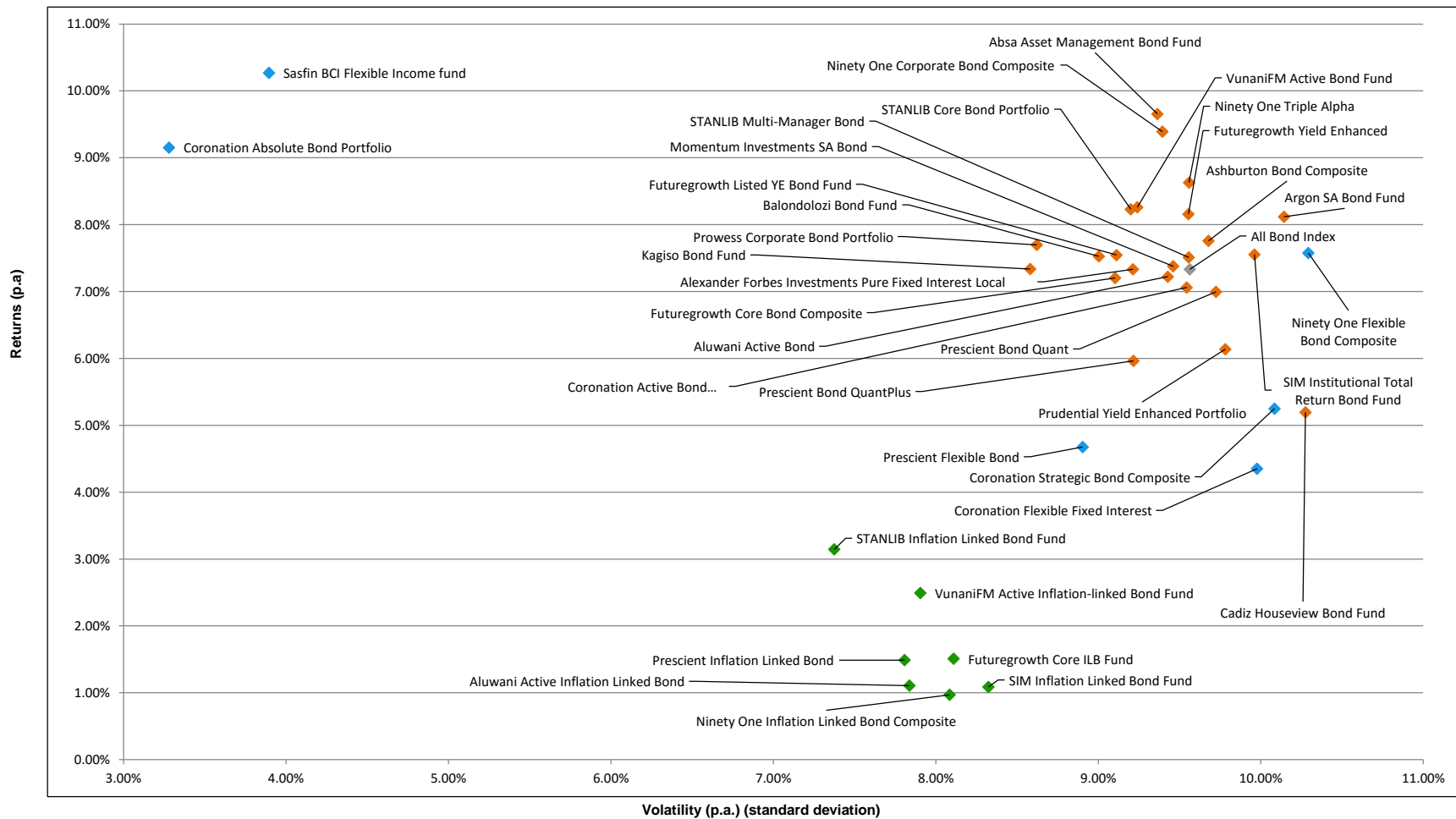
Volatility vs Return scatterplot – SA Bond Managers 3 Years ended 30 Sep 2020
