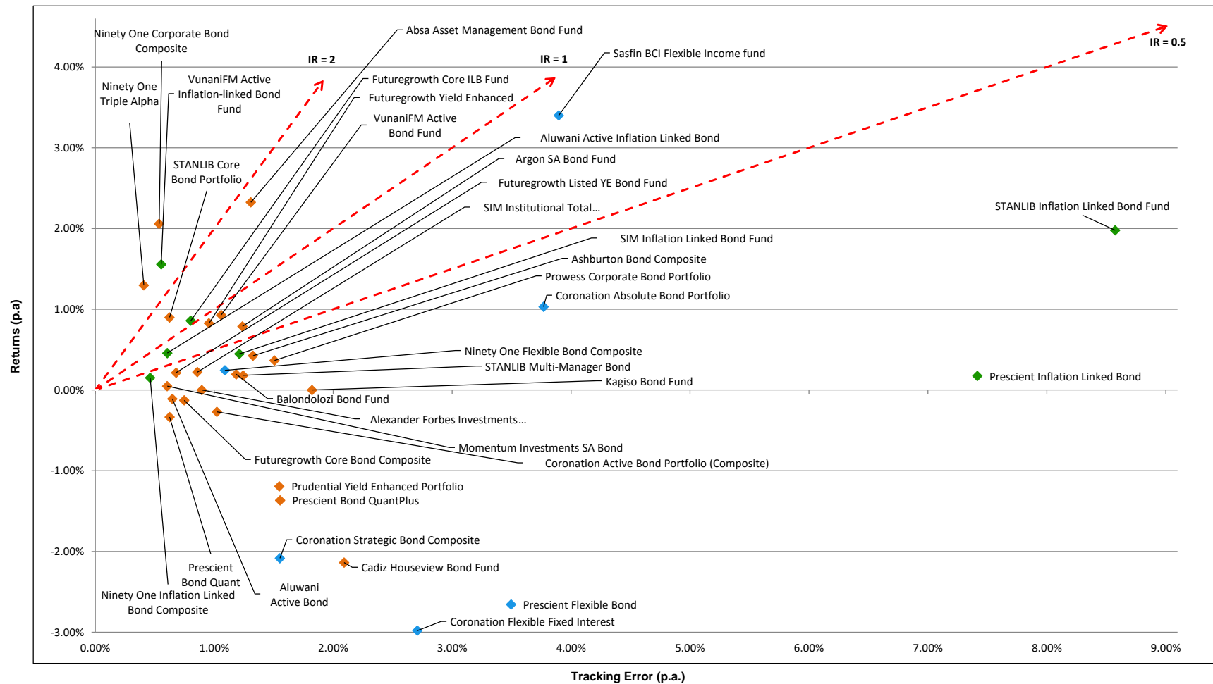
Active return vs Tracking Error scatterplot – SA Bond Managers 3 Years ended 30 Sep 2020
