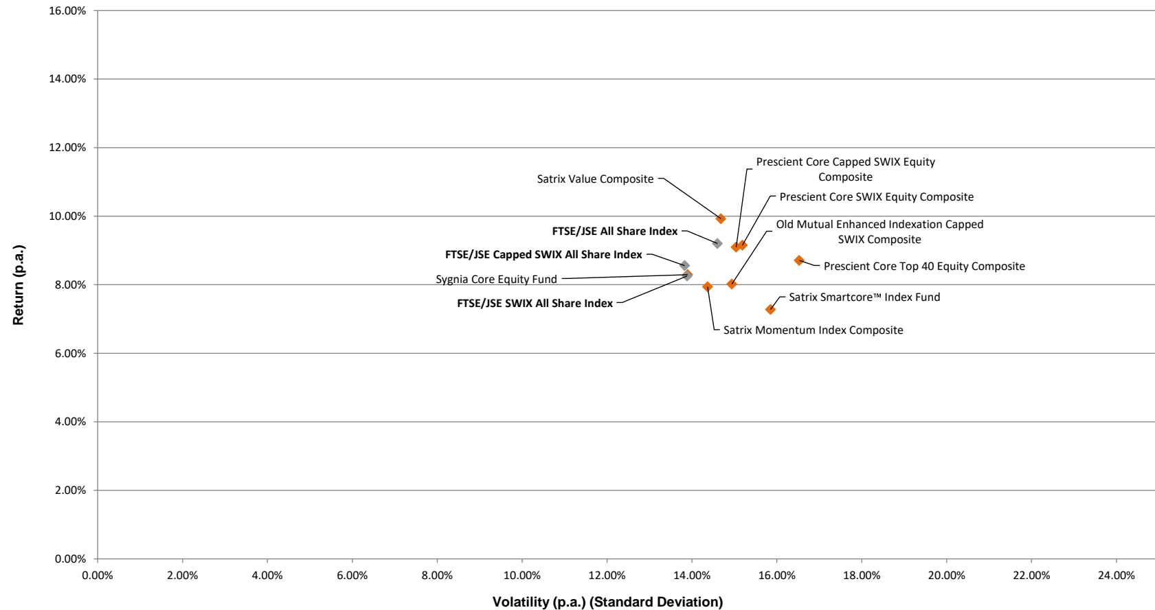
Risk vs Return Scatterplot on SA Equity Managers - Enhanced Index 3 years ended 31 January 2025
