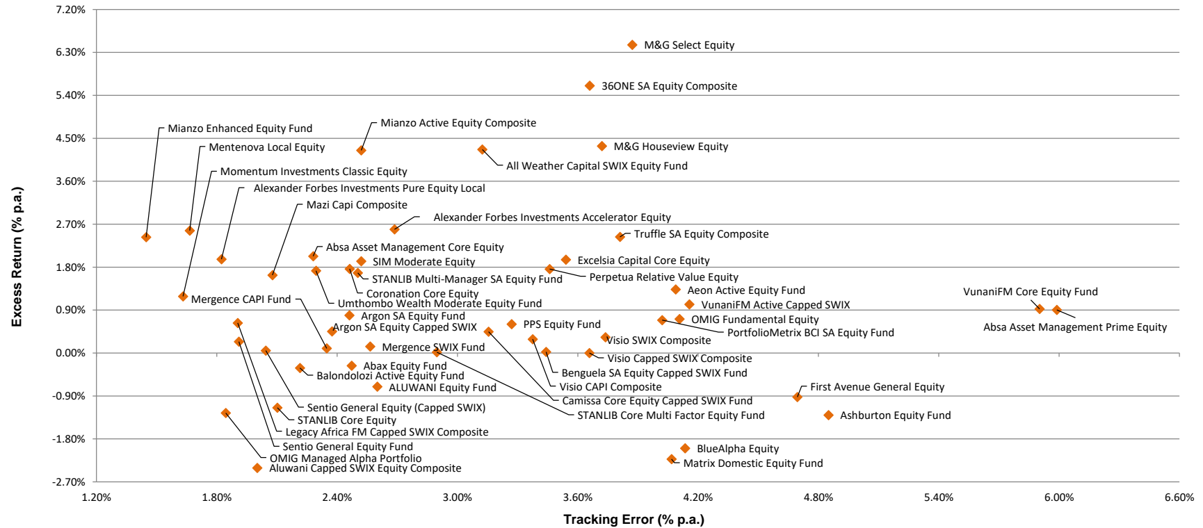
Excess Return vs Tracking Error Scatterplot - SA Equity Managers - Benchmark Cognisant 3 years ended 31 July 2023
