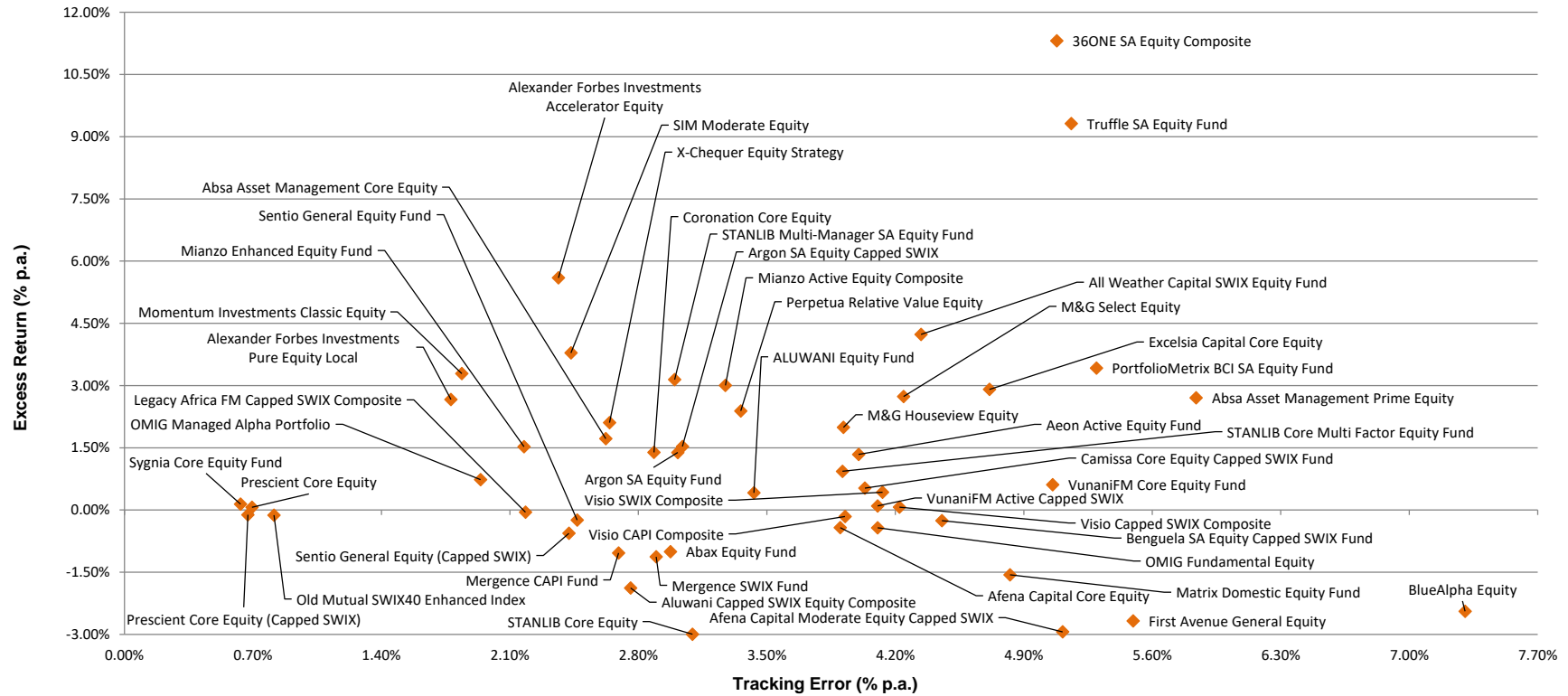
Excess Return vs Tracking Error Scatterplot - SA Equity Managers - Benchmark Cognisant 3 years ended 30 June 2022
