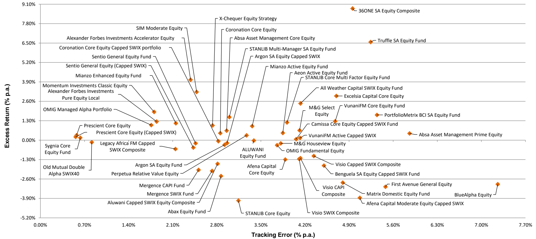
Excess Return vs Tracking Error Scatterplot - SA Equity Managers - Benchmark Cognisant 3 years ended 31 March 2022
