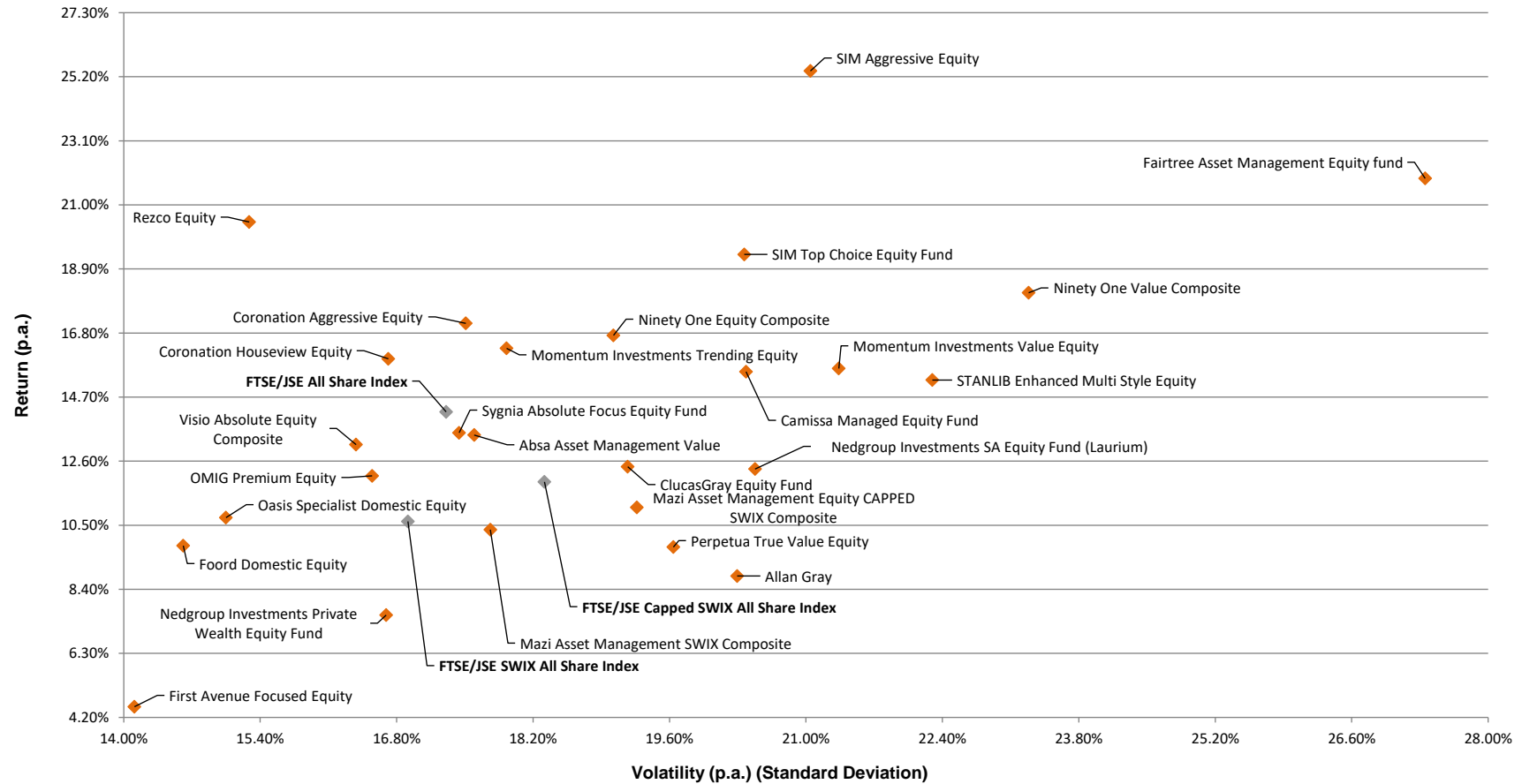
Risk vs Return Scatterplot on SA Equity Managers - Not Benchmark Cognisant 3 years ended 31 March 2022
