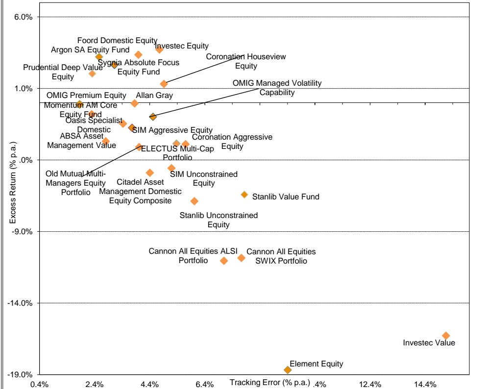
Excess return vs Tracking error Scatterplot - SA Equity Managers - Not Benchmark Cognisant 3 Years ended 30 September 2015
