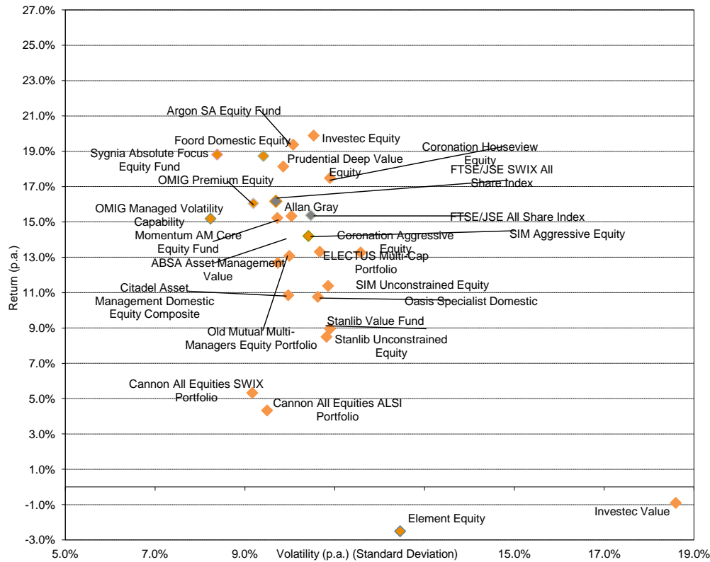
Risk vs Return Scatterplot on SA Equity Managers - Not Benchmark Cognisant 3 Years ended 30 September 2015
