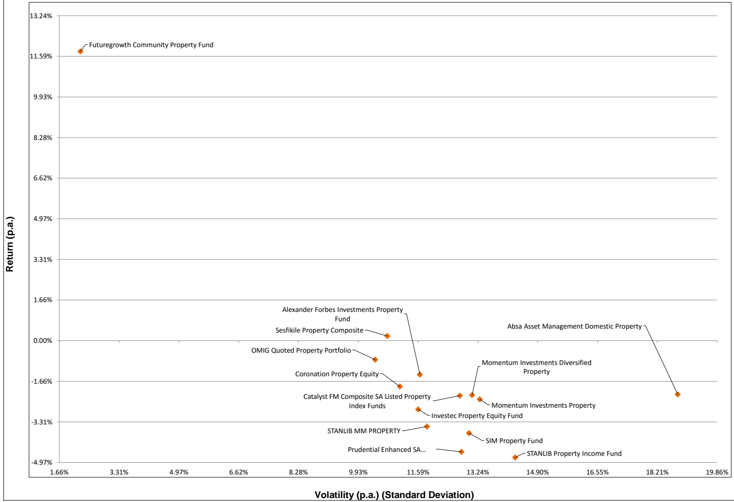
Volatility vs Return Scatterplot on Property Managers 3 Years ended 31 December 2019
