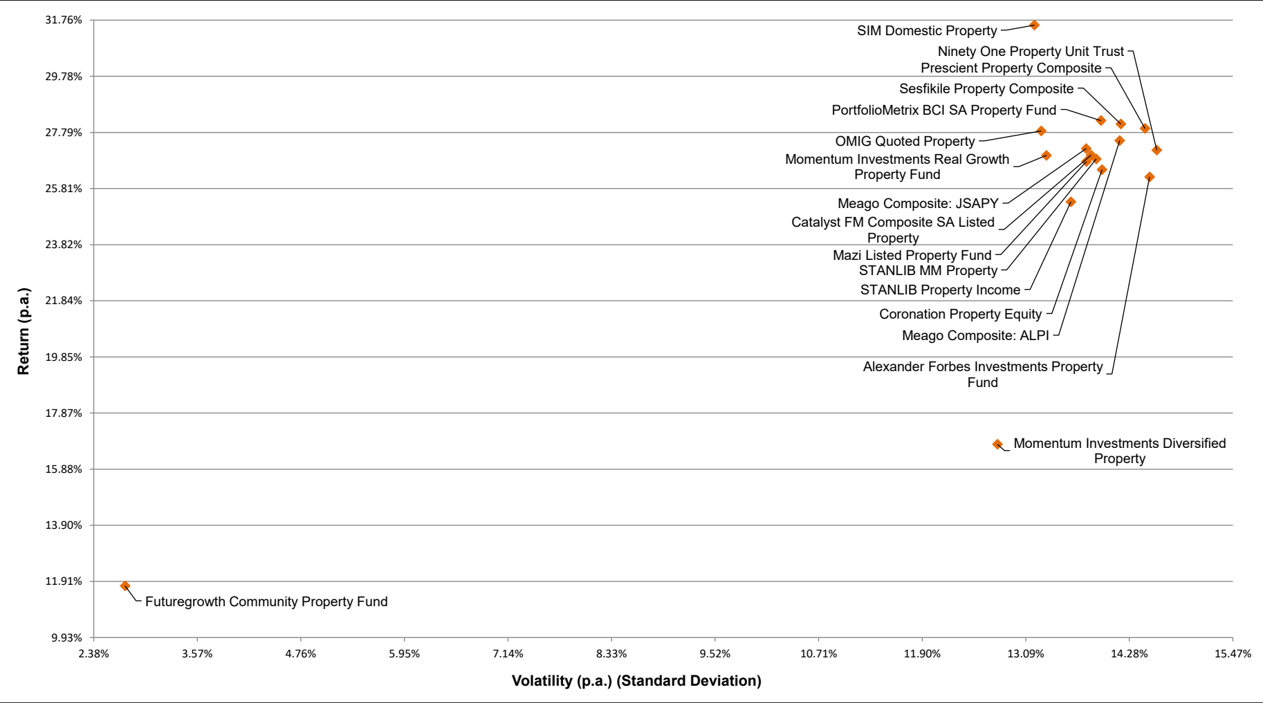
Volatility vs Return Scatterplot on Property Managers 3 Years ended 28 February 2026
