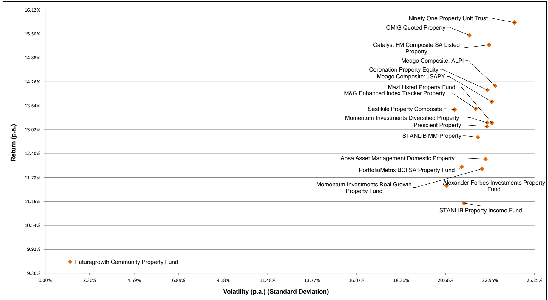
Volatility vs Return Scatterplot on Property Managers 3 Years ended 31 July 2023
