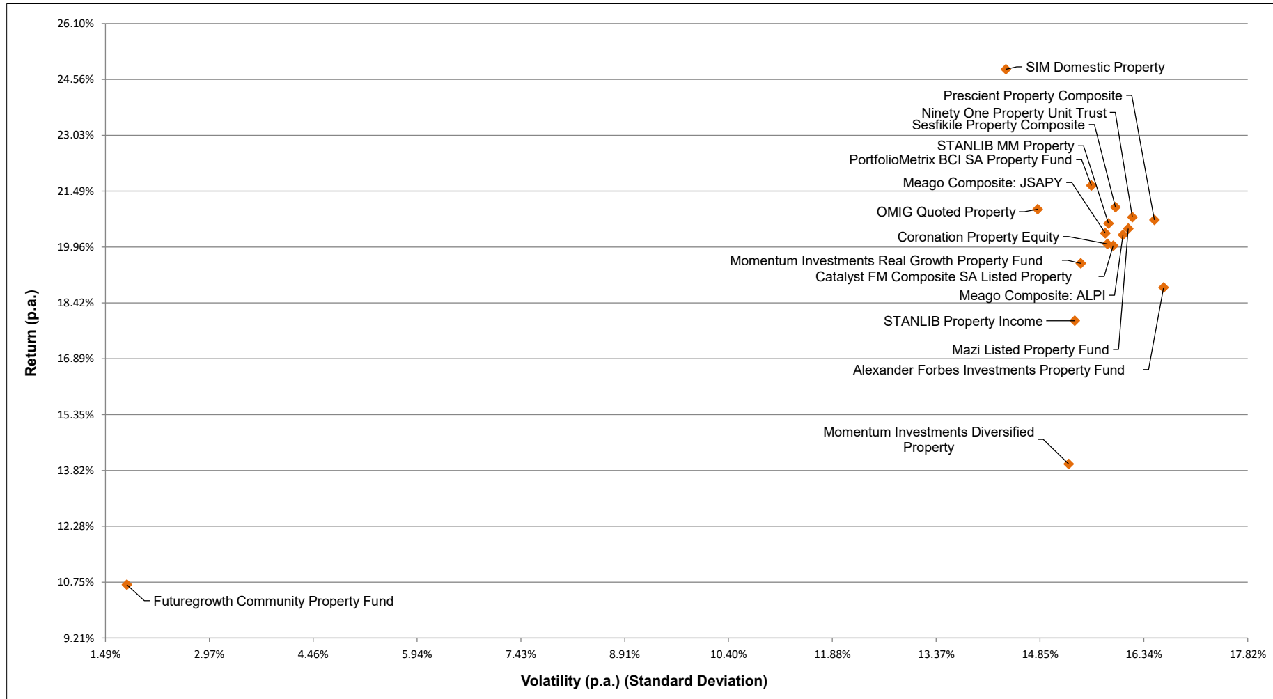
Volatility vs Return Scatterplot on Property Managers 3 Years ended 30 June 2025
