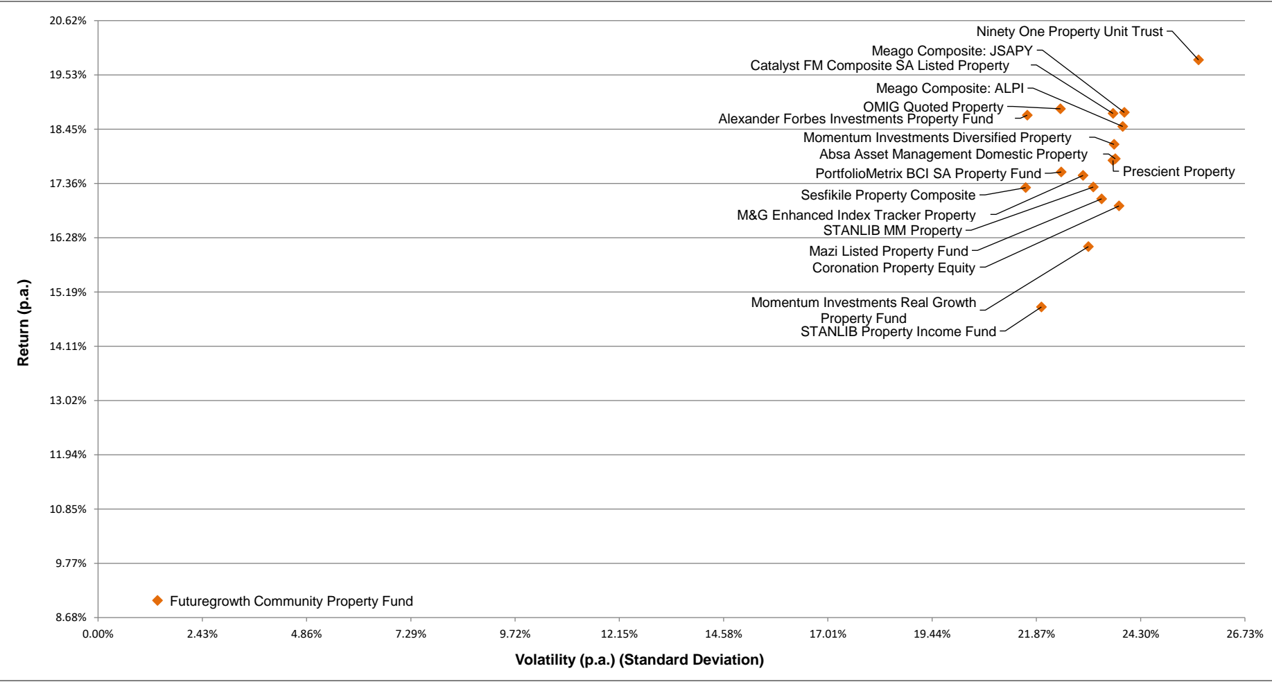
Volatility vs Return Scatterplot on Property Managers 3 Years ended 31 March 2023
