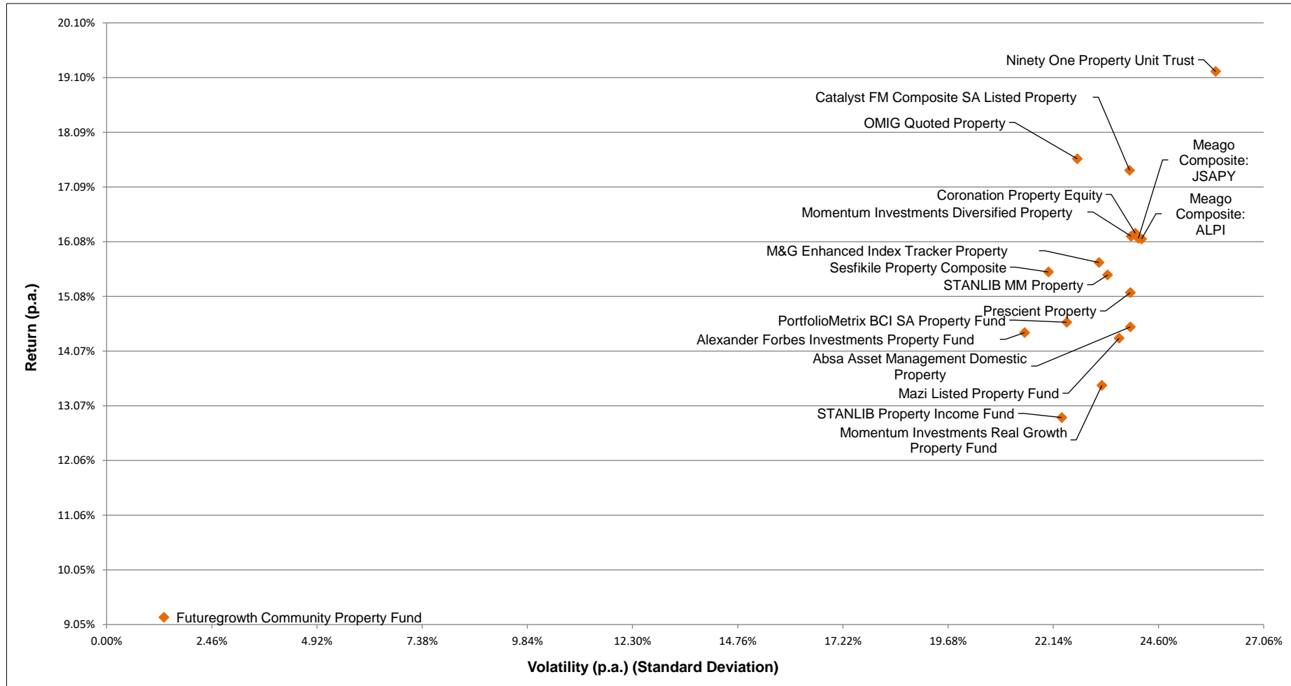
Volatility vs Return Scatterplot on Property Managers 3 Years ended 31 May 2023
