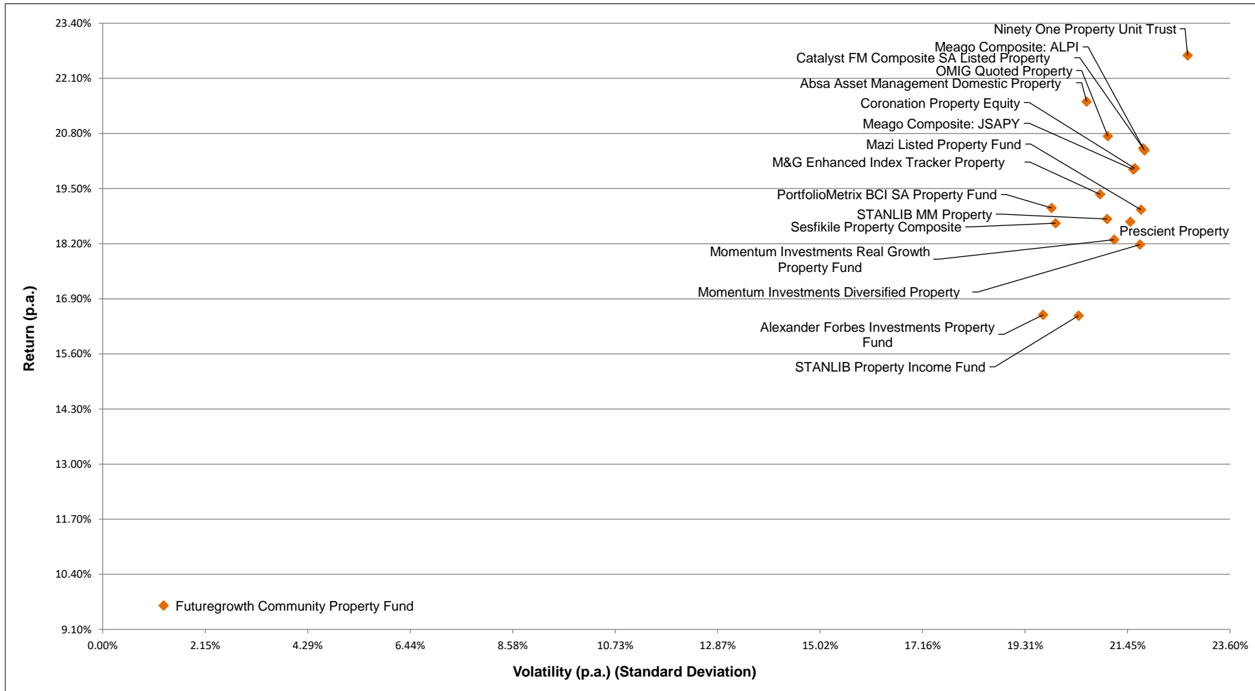
Volatility vs Return Scatterplot on Property Managers 3 Years ended 31 October 2023
