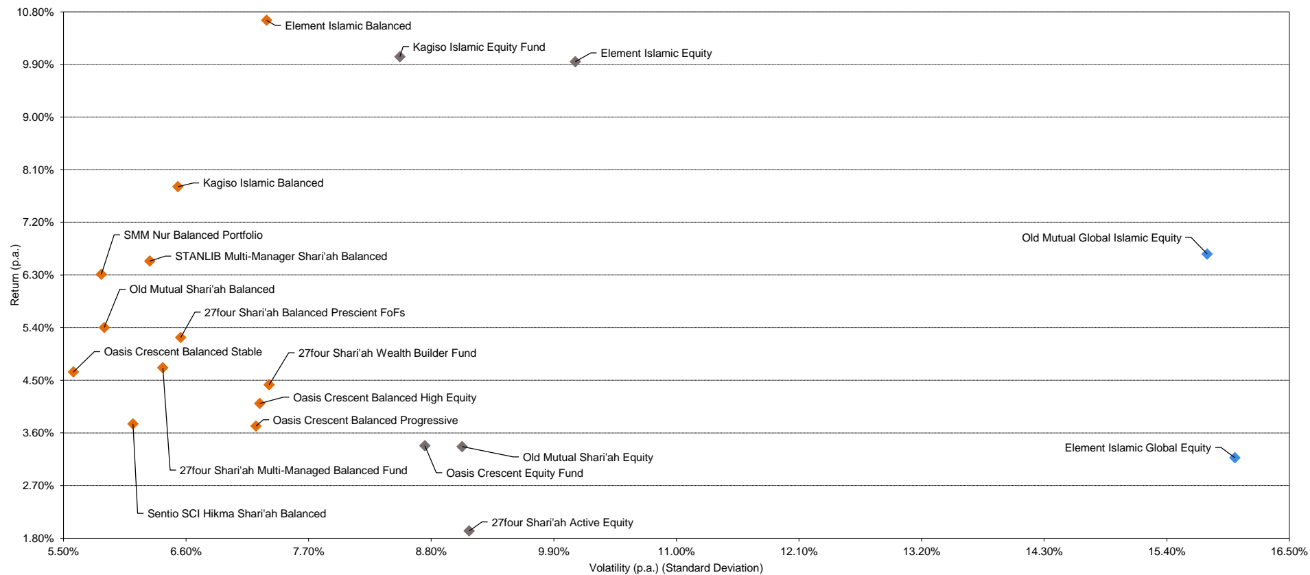
Risk vs Return Scatterplot on Shari'ah Compliant Portfolios - Balanced and Equity mandates 3 Years ended 30 June 2019
