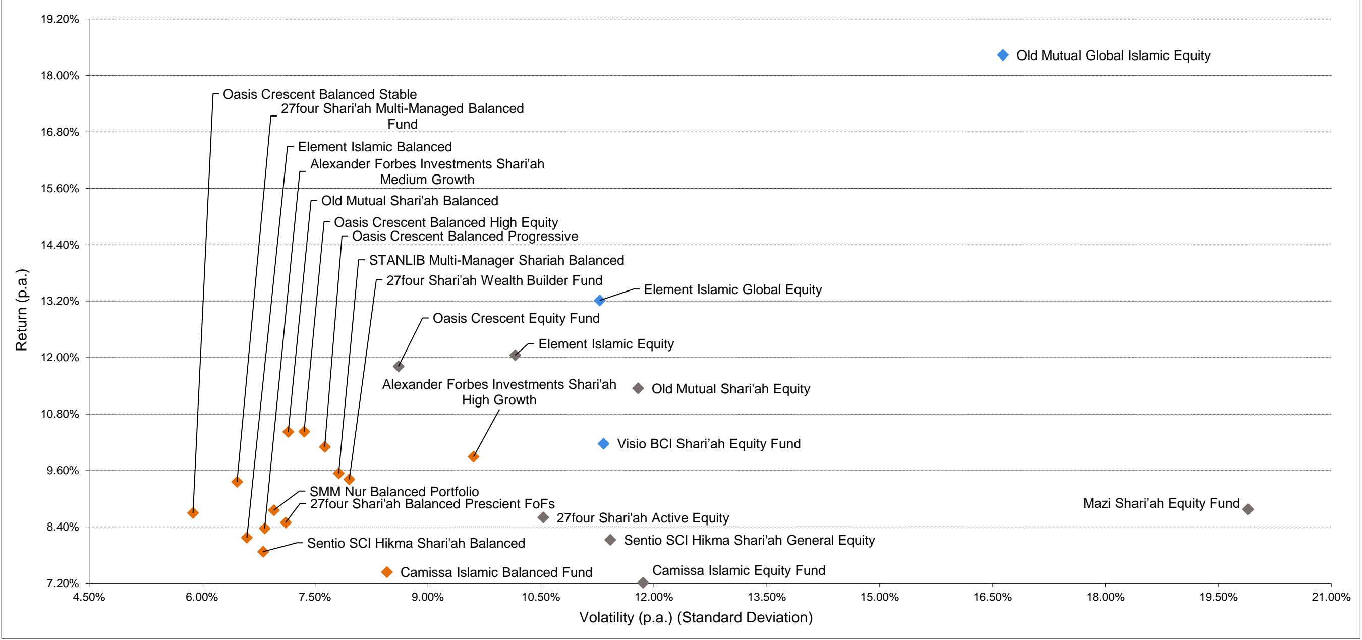
Risk vs Return Scatterplot on Shari'ah Compliant Portfolios - Balanced and Equity mandates 3 Years ended 30 June 2024
