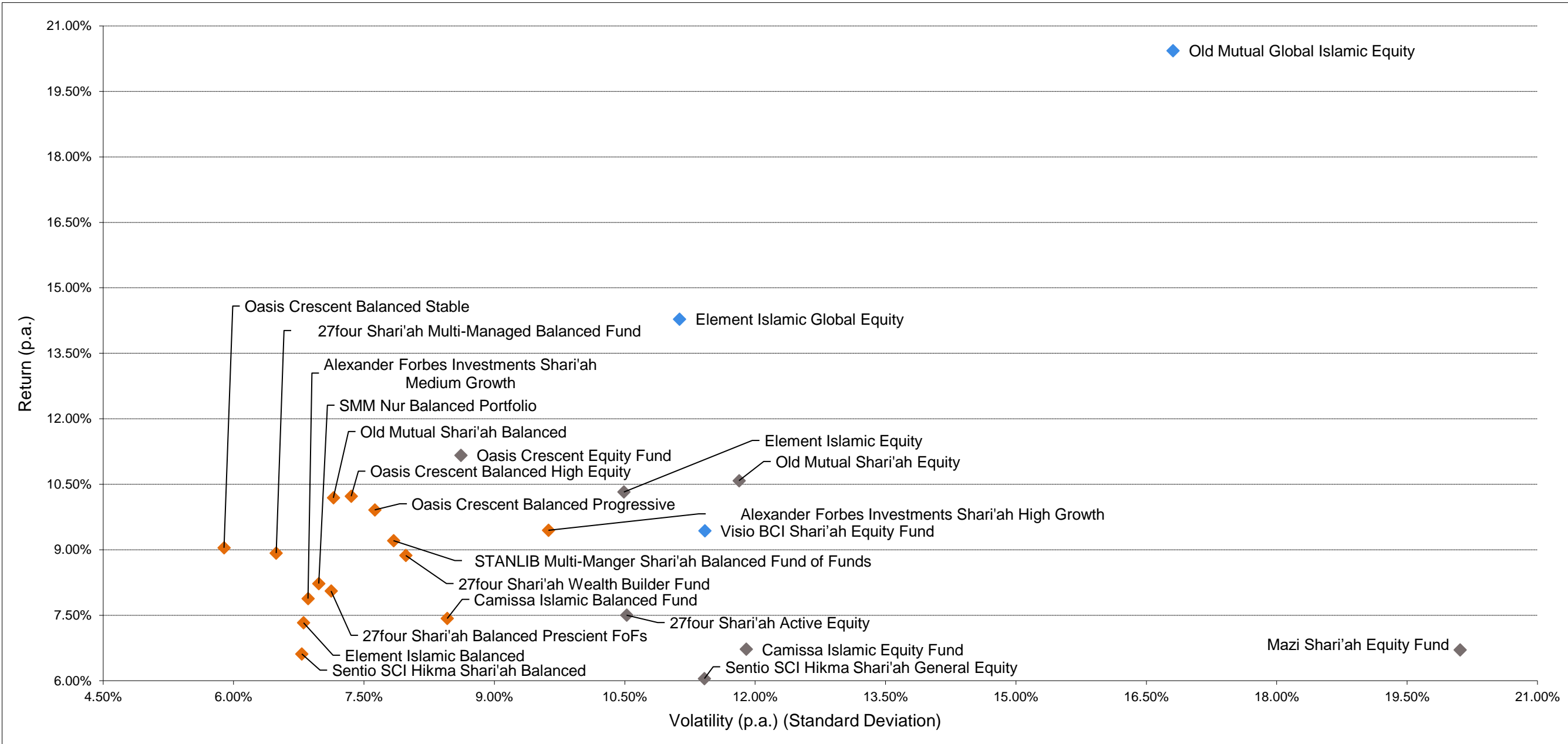
Risk vs Return Scatterplot on Shari'ah Compliant Portfolios - Balanced and Equity mandates 3 Years ended 31 May 2024
