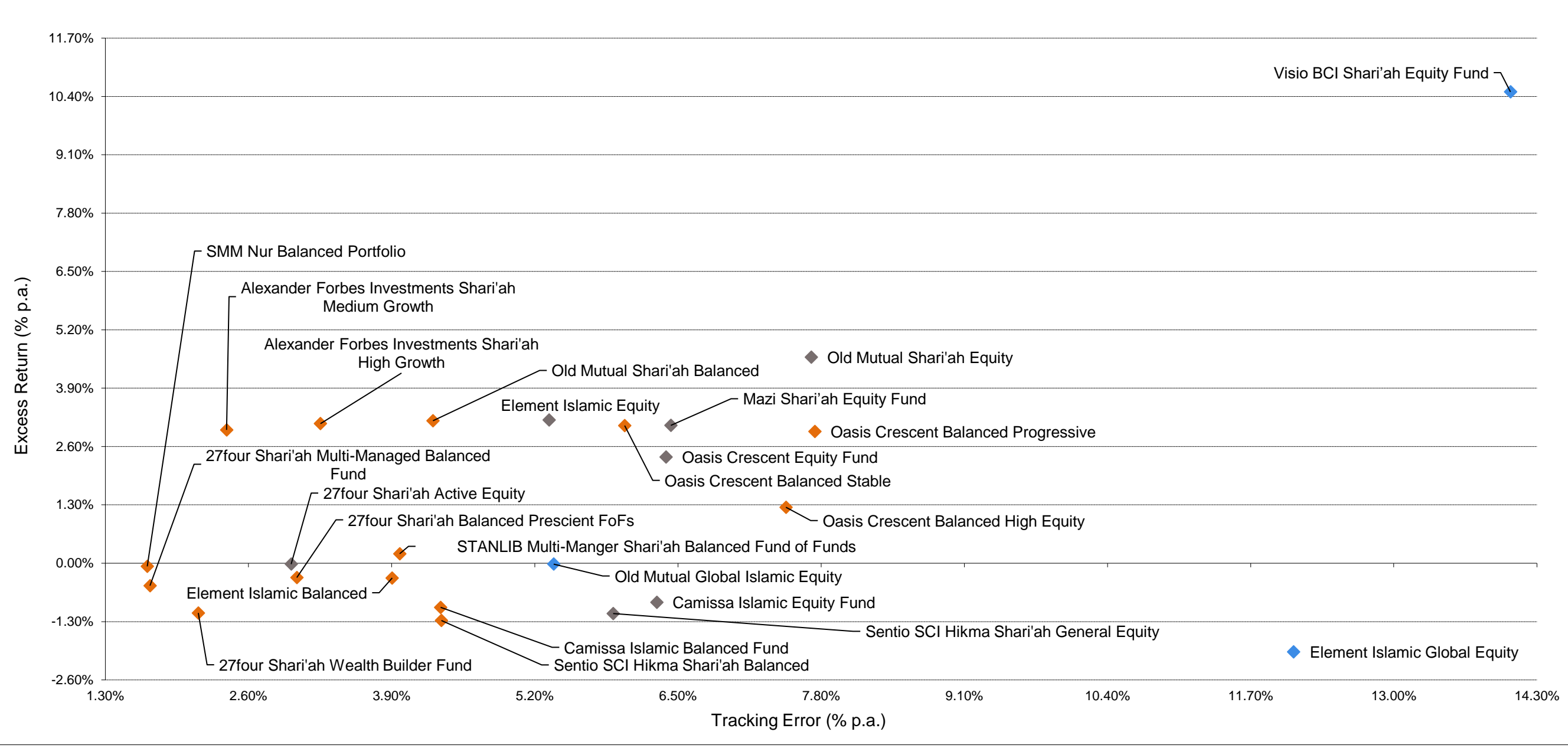
Excess Return vs Tracking Error Scatterplot - Shariah Compliant Portfolios - Balanced and Equity mandates 3 Years ended 31 May 2024
