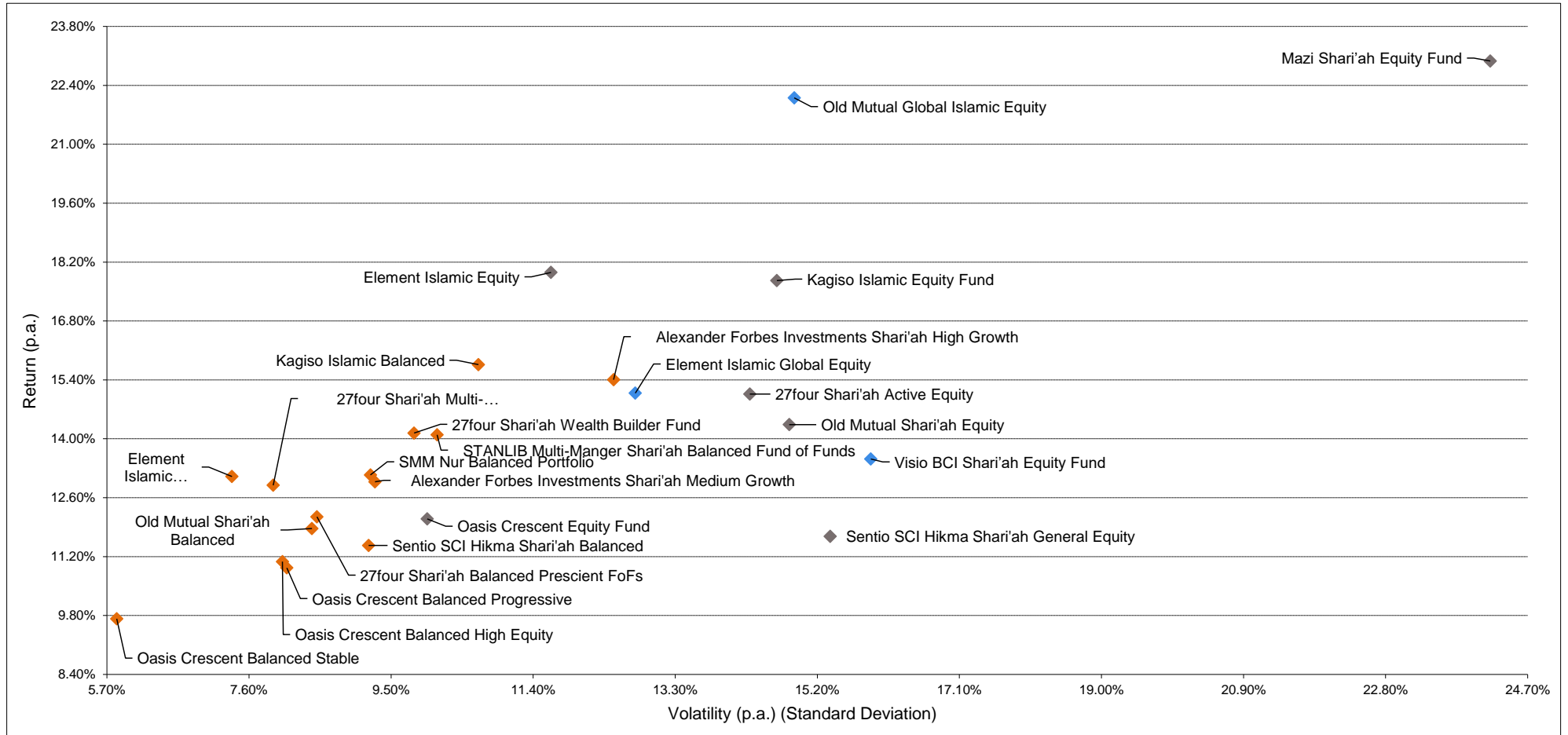
Risk vs Return Scatterplot on Shari'ah Compliant Portfolios - Balanced and Equity mandates 3 Years ended 30 November 2021
