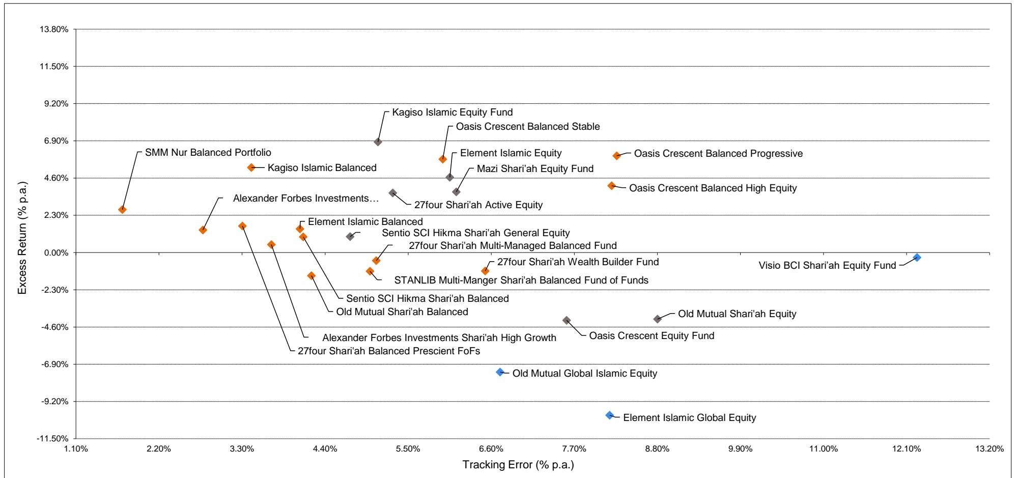
Excess Return vs Tracking Error Scatterplot - Shariah Compliant Portfolios - Balanced and Equity mandates 3 Years ended 30 November 2021
