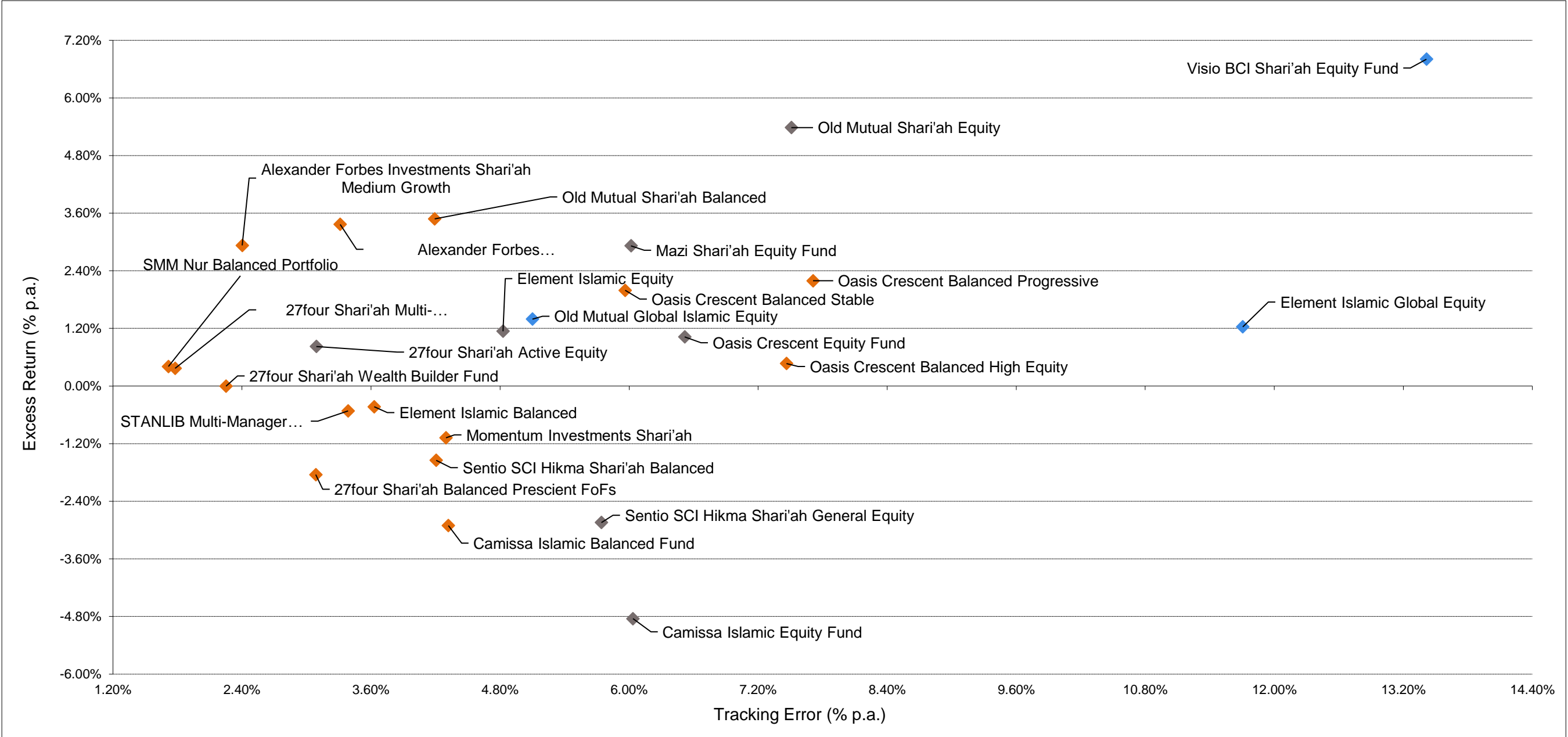
Excess Return vs Tracking Error Scatterplot - Shariah Compliant Portfolios - Balanced and Equity mandates 3 Years ended 30 September 2024
